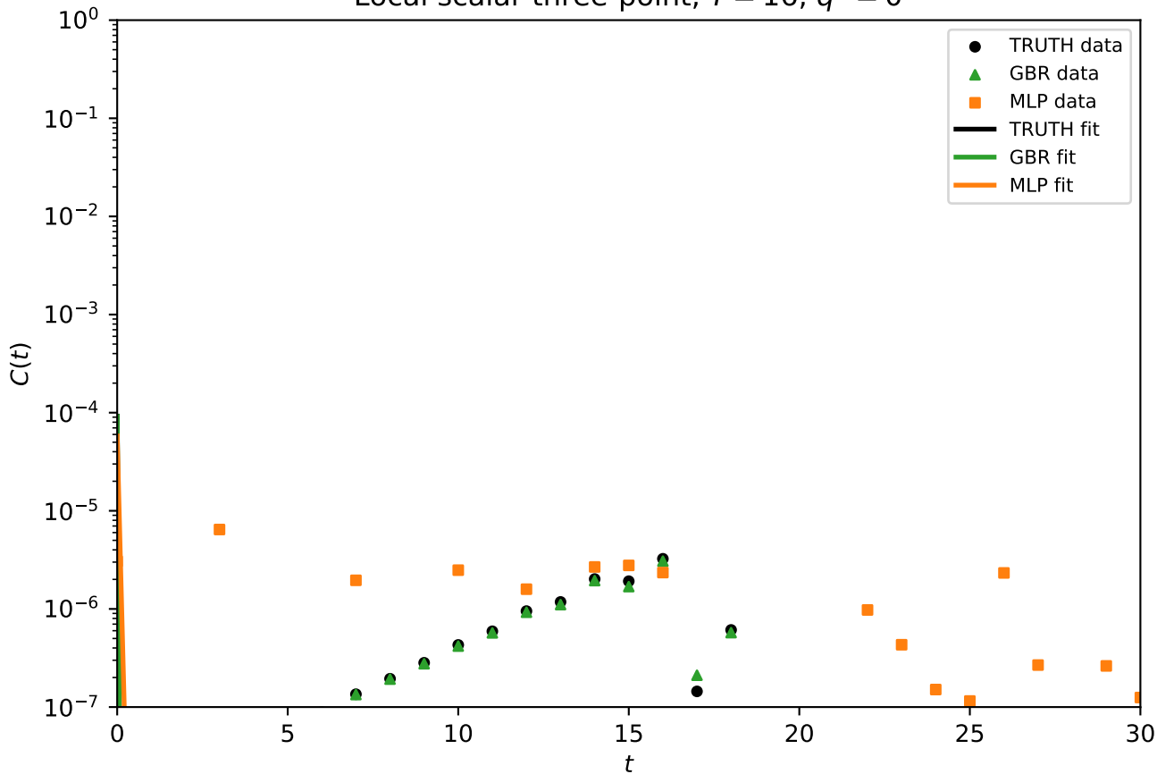
Local scalar three-point, T = 16 , q^2 = 0
